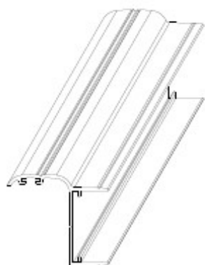
Couvre joint
